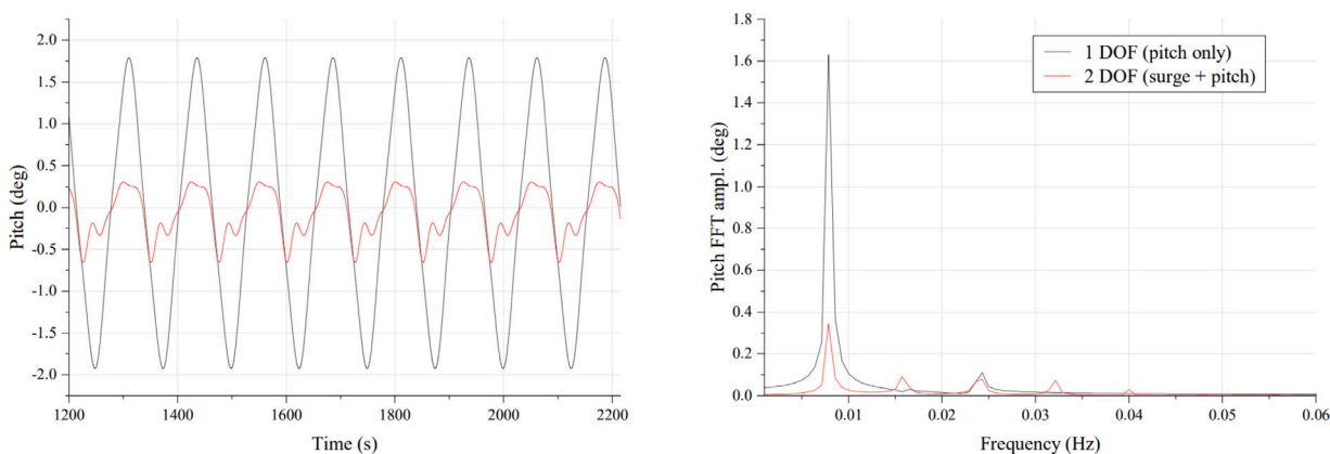
Fig. 17. A comparison of pitch motion time history and FFT amplitudes in a 2 DOF coupled motion against a 1 DOF uncoupled motion.
