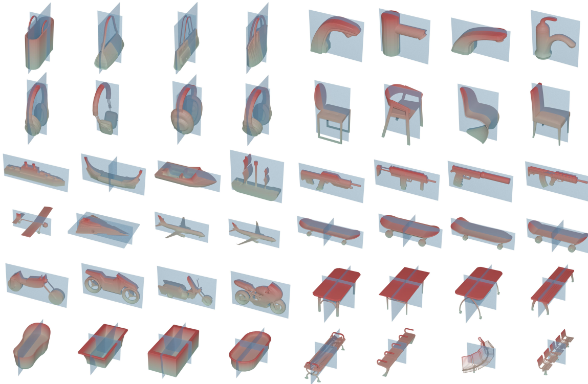
Figure 3: Qualitative results for reflective symmetry detection on the test set of ShapeNet [2]. From left to right, top to bottom are of the categories: bag, water tap, earphone, chair, boat, rifle, airplane, skateboard, motorcycle, table, bathtub and bench. 4 instances are displayed for each category. Our method is able to detect multiple symmetry planes accurately. For better visualization, we paint the shapes with gradient color.
