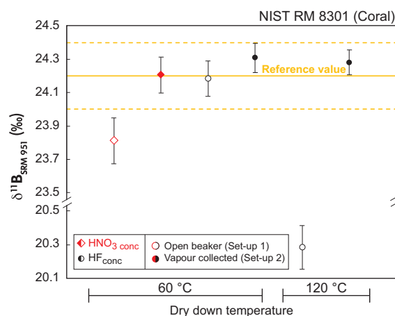
Figure 5. \delta^{11}\text{B}_{\text{SRM } 951} of synthetic coral isotope reference material (NIST RM 8301 (Coral)), that was dried to convert from strong HF or \text{HNO}_3 acid to 0.5 \text{ mol l}^{-1} \text{HNO}_3 , simulating the dissolution procedure. The dashed yellow lines represent the 2s variability of the interlaboratory consensus value, Stewart et al. (2020). Open circles denote samples where vapour was allowed to escape rapidly during the drying process (uncovered beakers), while filled circles represent samples where evaporation was carried out in a semi-enclosed environment (see Figure 1). Red symbols indicate \text{HNO}_3 acid matrix, black symbols indicate HF acid matrix.
