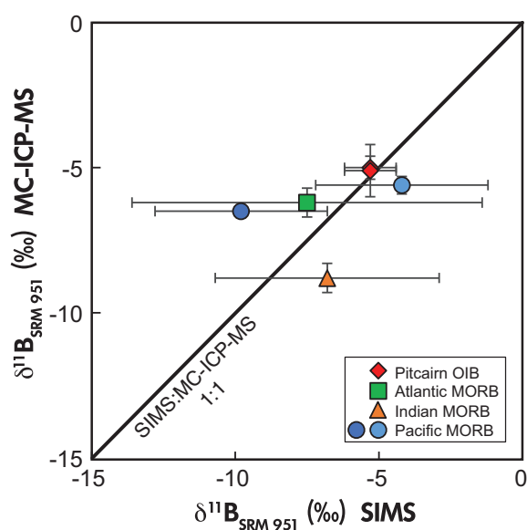
Figure 4. \delta^{11}\text{B}_{\text{SRM } 951} of volcanic glass obtained by in situ SIMS (x-axis, Marschall et al. 2017) and MC-ICP-MS using HF digestion (y-axis) in this study ( 2s range bars shown). Samples with higher boron mass fraction ( \geq 2 \mu\text{g g}^{-1} ) exhibit better correlation between SIMS and MC-ICP-MS data (Pitcairn OIB).
