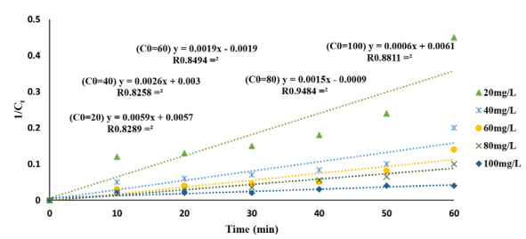
Fig. 11. Pseudo Second-Order Plot for Cephalexin Removing Using the UV/MgO/GAC System.
