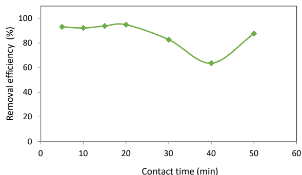
Fig. 5. Effect of Contact Time on the Removal of MB. (Nanoparticle dosage: 0.05 g/L, initial MB concentration: 40 mg/L, pH: 5, \text{H}_2\text{O}_2 concentration: 2 g/L)
