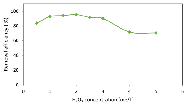
Fig. 4. Effect of \text{H}_2\text{O}_2 Concentration on the Removal of MB. (Nanoparticle dosage: 0.05 g/L, initial MB concentration: 40 mg/L, pH: 5, contact time: 20 minutes)
