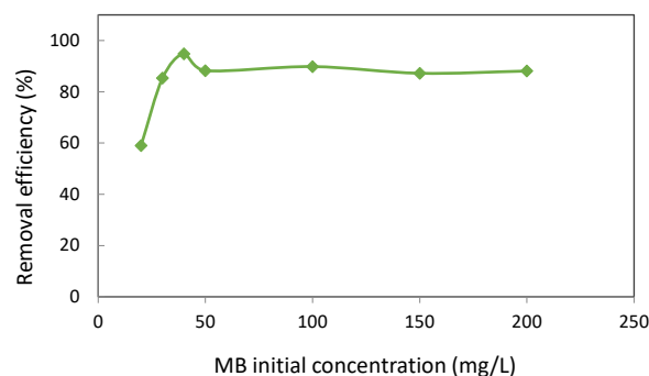
Fig. 1. Effect of Different Concentrations of Methylene Blue on Removal Efficiency. (Nanoparticle dose: 0.05 g/L, pH: 5, contact time: 20 minutes, H_2O_2 concentration: 2 mg/L)
