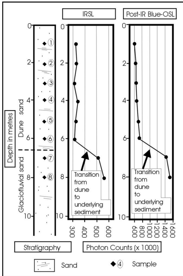
Figure 4 Stratigraphy and luminescence profiles (IRSL and post- IR blue OSL) for site NS01.
