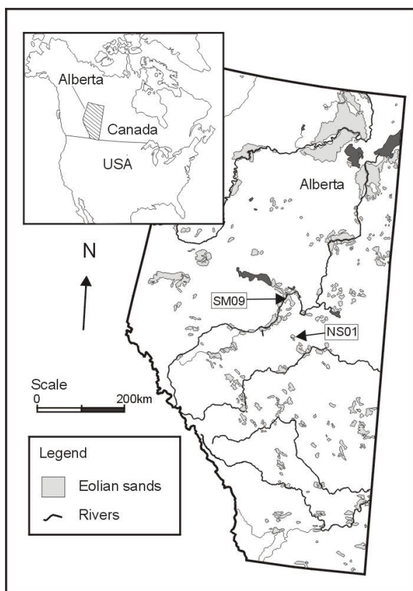
Figure 2 Study area in central Alberta showing sites SM09 (Hondo dune field) and NS01 (Nestow dune field).
