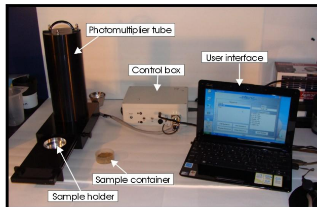
Figure 1 Basic components of a portable OSL reader system.
