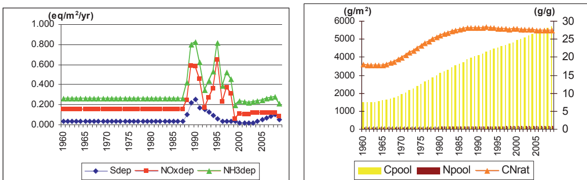
Figure BG.3 Results of the dynamic modeling - VSDp for Vitinya site for the period 1960 - 2010
