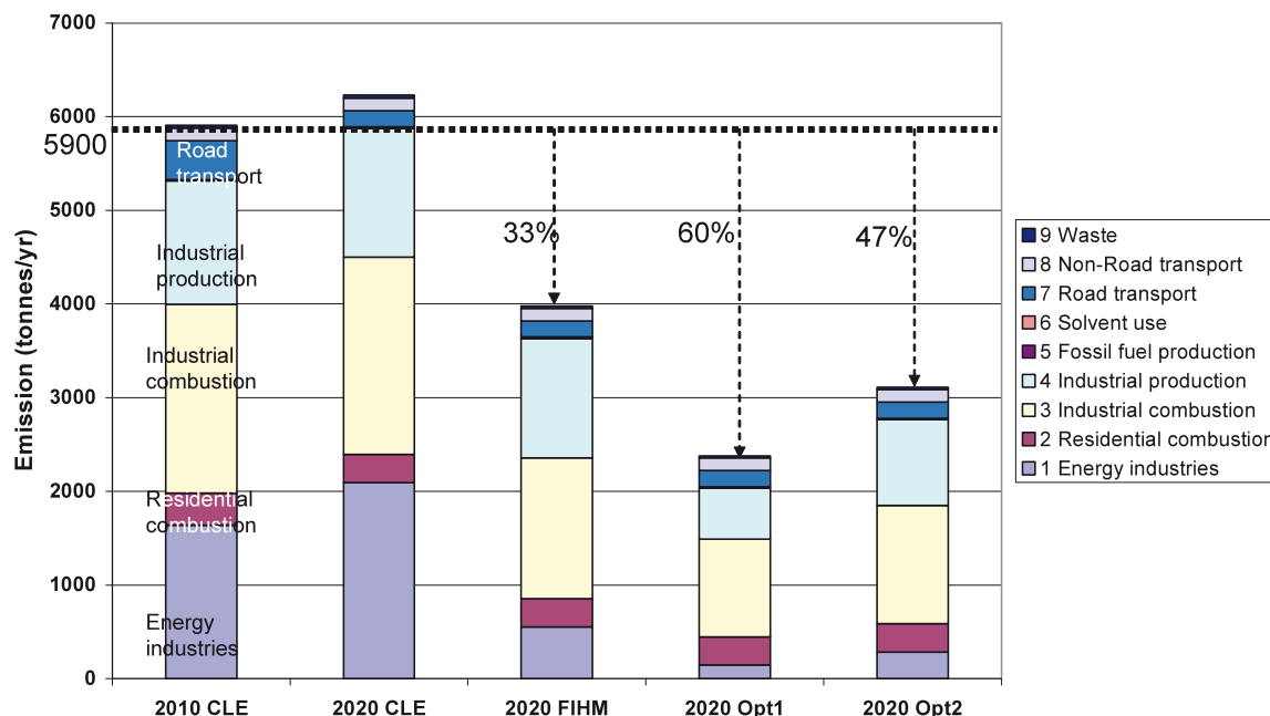
Figure 6.2 Pb emissions per sector, and the reductions under the four scenarios.
