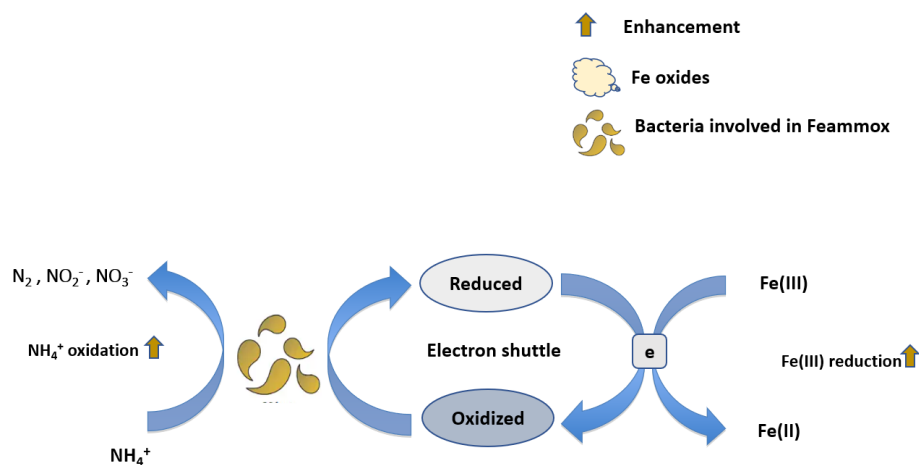
Figure 4. Electron shuttles enhance Fe reduction and NH 4 + oxidation (Feammox) rates.
