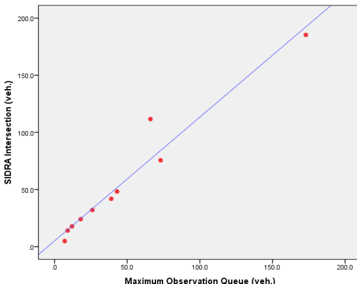
Figure 4: Comparison of queue vehicles estimated by SIDRA Intersection 6.0 with MOQ.
