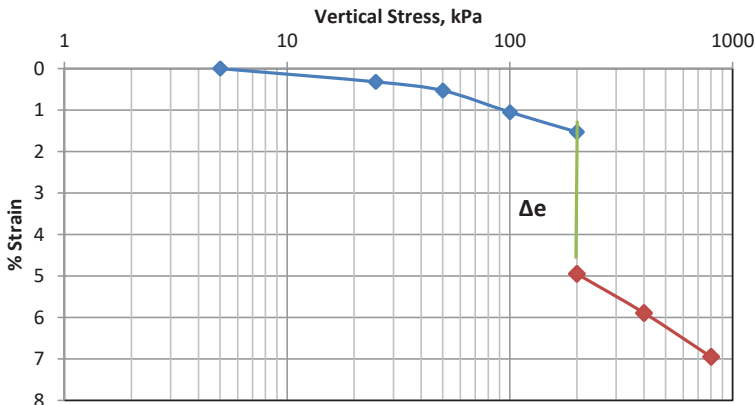
Figure 7: Findings of the untreated soil collapse test.
