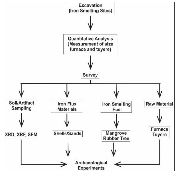
Figure 3. Archaeological experiment flow chart of iron smelting at the SBAC (Source: Research data analysis, 2023)
