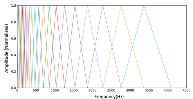
FIGURE 3. Mel frequency window bank.
