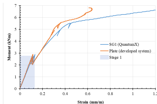
Figure 17. Moment vs. strain diagram for beam VT2.
