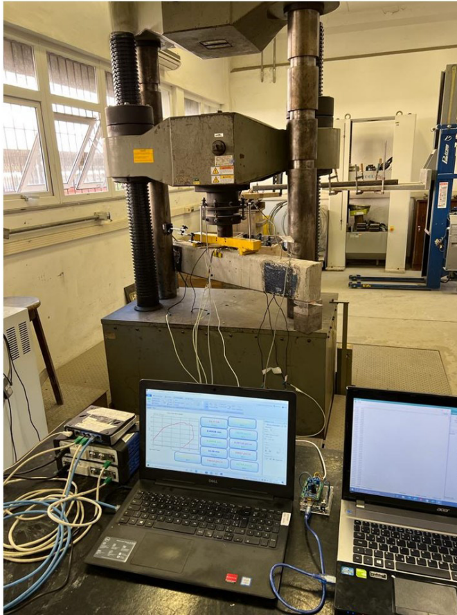
Figure 10. Test setup.
