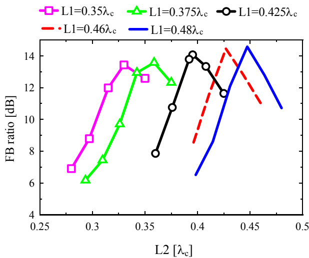
Fig. 3 Maximum front-to-back ratio
