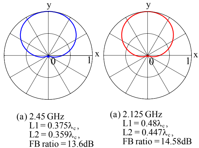
Fig. 6 Electric field radiation patterns in xy plane
