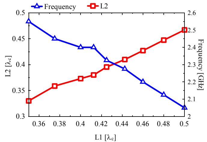
Fig. 4 L2 for maximum FB ratio and its frequency
