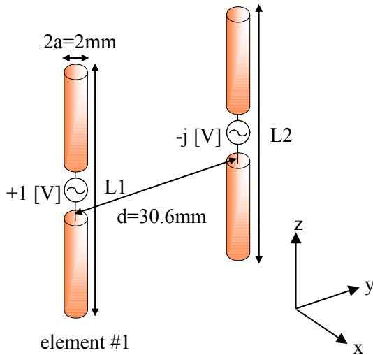
Fig. 1 Analytical model
