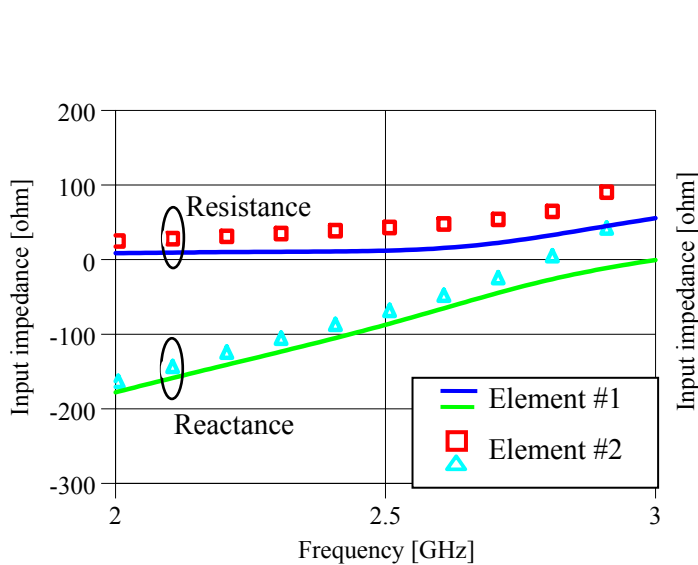
Fig. 8 Calculated input impedances at feed points of each element. L1=0.375 \lambda_c , L2=0.359\lambda_c .
