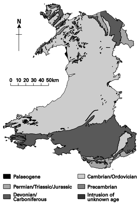
Fig. 2 Outline geology of Wales
