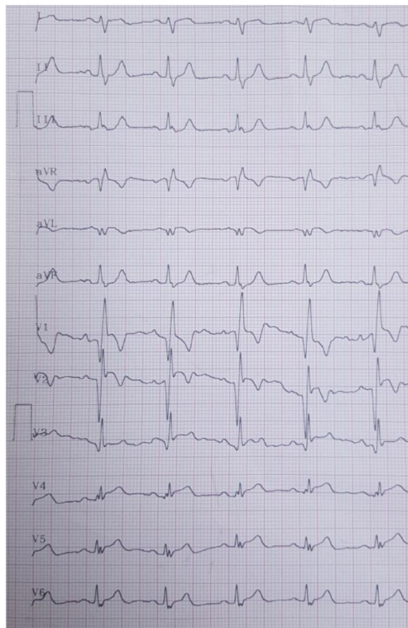
Figure 1. Electrocardiography
