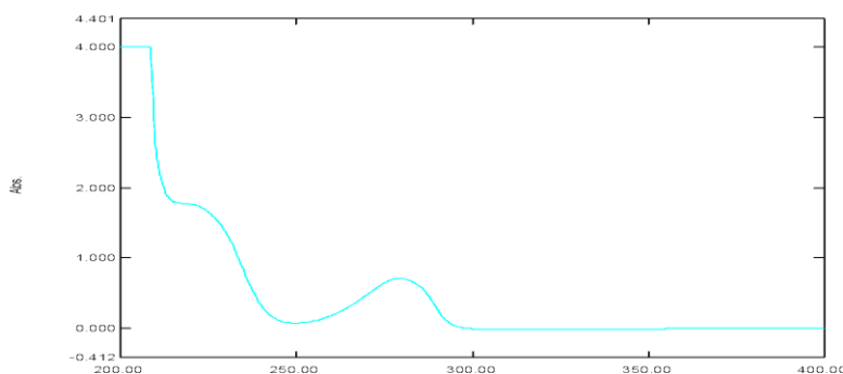
Figure No. 2: \lambda_{\text{max}} of Norepinephrine
