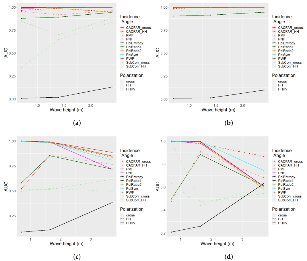
Figure 12. Comparison of the detector AUCs for different wave heights for HV HH. (a) Wind: up/down, incidence angle: medium and boat orientation: 45°. (b) Wind: up/down, incidence angle: medium and boat orientation: 90°. (c) Wind: up/down, incidence angle: high and boat orientation: 45°. (d) Wind: up/down, incidence angle: high and boat orientation: 90°.
