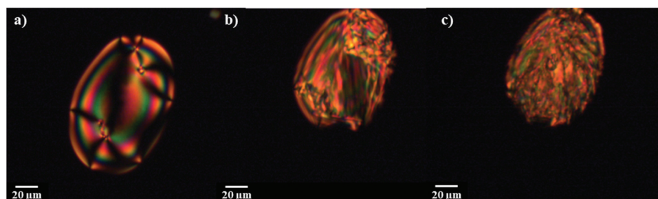
Figure 3. (Colour online) The optical textures seen for isolated droplets of CB7SS7CB in the (a) nematic ( T = 94^\circ\text{C} ), (b) twist-bend nematic ( T = 40^\circ\text{C} ) and (c) crystal phases ( T = 38^\circ\text{C} ).
