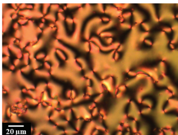
Figure 2. (Colour online) The schlieren texture of the nematic phase shown by CB6SS6CB ( T = 77^\circ\text{C} ).
