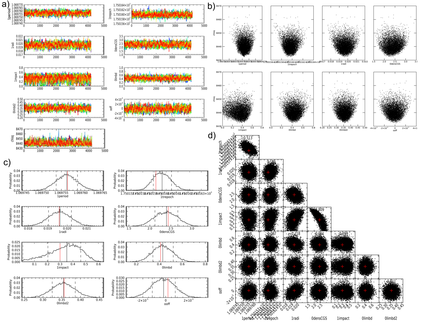
Fig. C.1: Graphical output from MCMC sequence performed by UFIT that led to the results reported in Table 7. In all panels, the parameters are indicated by the keywords used in UFIT: “1period” for the planet period, “1trepoch” for the epoch of transit, “1radi” for the relative planet radius, “0densCGS” for the stellar density in CGS units, “1impact” for the impact parameter, “0limbd” and “0limbd2” for the LD coefficients q_1 and q_2 , and “ooff” for the off-transit flux-offset against zero. The sub-figures are: (a) Values of the parameters against link-number of the MCMC sequence, excluding burn-in. Each MCMC chain is shown by a different color. The lowest panel shows the evaluation of the \chi^2 values. (b) Scatter plot of parameters versus the \chi^2 value. (c) Histograms of parameter distributions. The median value is shown by the vertical black line; the dashed lines delimit the 68.3% credible interval and the red line gives the value of the best fit. (d) Corner plot of the correlations among parameters. The red crosses give the values of the best fit.
