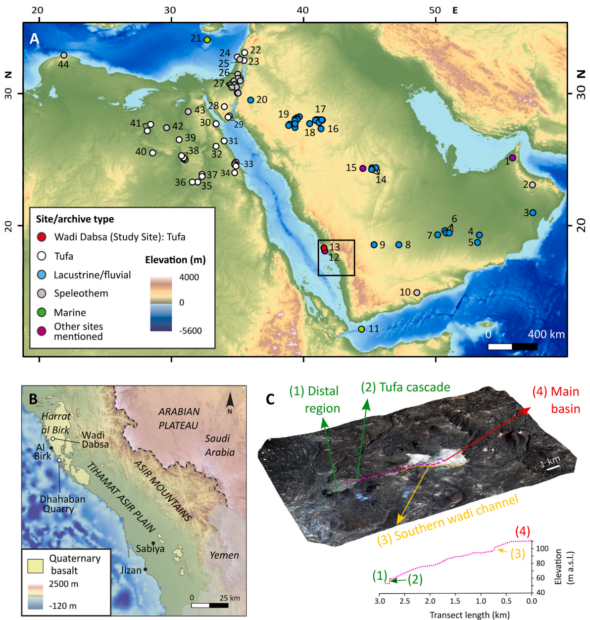
Fig. 1. (A) Location map showing sites of palaeoenvironmental records for the late Pleistocene on the Arabian Peninsula, the Levant and Palestine/Israel, and into western North Africa, as well as other sites mentioned in the text, alongside the location of the Wadi Dabsa study site, noting that the Tadrart Acacus (tufa site) in Libya is out of view, further west. See Supp. Info 1 for corresponding site names. Topographic and bathymetric data from GEBCO Compilation Group, 2022 , (B) Location of the Harrat al Birk on the Tihamat Asir Plain on south-western Saudi Arabia (adapted from Inglis et al., 2019 ), (C) Dabsa Basin, indicating the four key locations of investigated tufa (surface of the main basin, southern wadi channel, tufa cascade and distal region), on an ASTER 30 m GEDM, with 3x vertical exaggeration using Pleiadas 1 Multispectral true colour scheme) (adapted from Inglis et al. (2019) ). See Supp. Info. 2 for detailed information about field locations of each sample at Wadi Dabsa and photographs.
