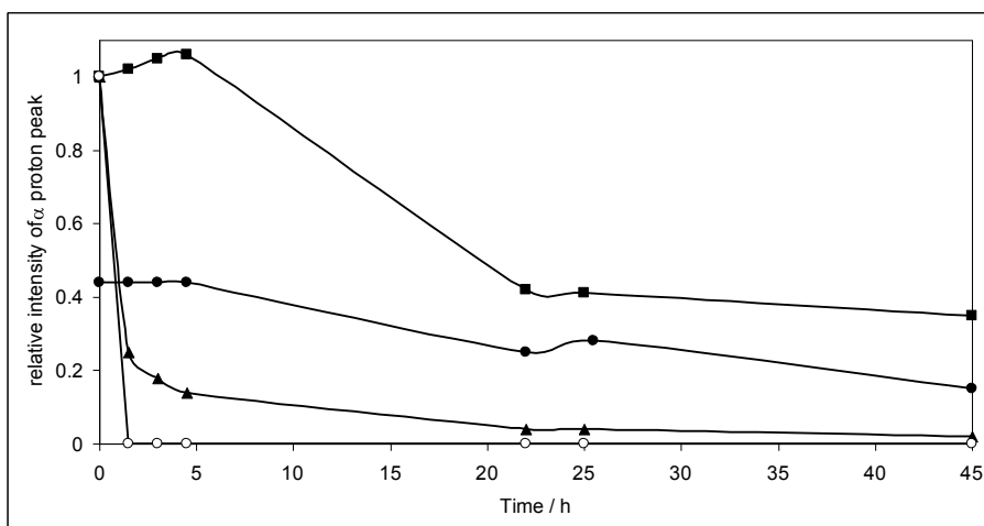
Figure 3: Plot of \alpha ^1\text{H} resonance intensity as a function of time in DMAP stabilised Pd nanoparticle dispersions. (■) dispersion at room temperature, (▲) dispersion held at 50 °C, (○) Dispersion held at 80 °C, (●) dispersion held at 50 °C with extra DMAP added following 25 h of H-D exchange- see text for details.
