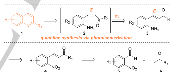
Scheme 1. Synthesis route towards quinoline targets.
