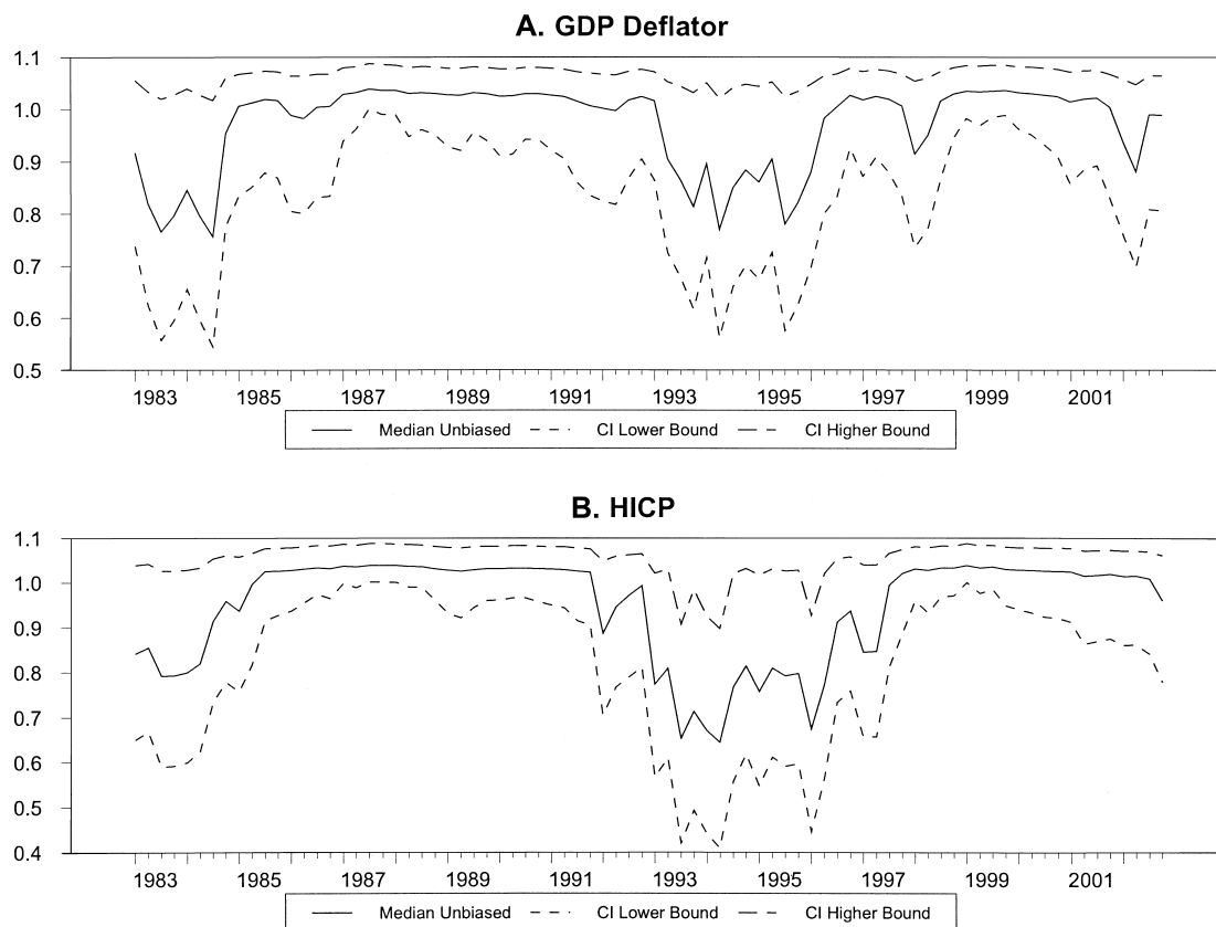
FIGURE 6.—ROLLING 12-YEAR ESTIMATES OF LARGEST AUTOREGRESSIVE ROOT (WITH 90% CONFIDENCE INTERVAL)
