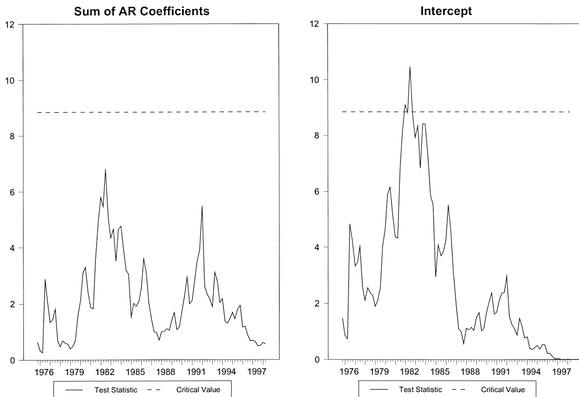
FIGURE 2.—CHOW TEST SEQUENCES AND 5% CRITICAL VALUES: UNIVARIATE MODEL
