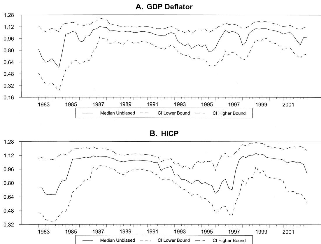
FIGURE 4.—ROLLING 12-YEAR GRID-BOOTSTRAP ESTIMATES OF \rho (WITH 90% CONFIDENCE INTERVALS)
