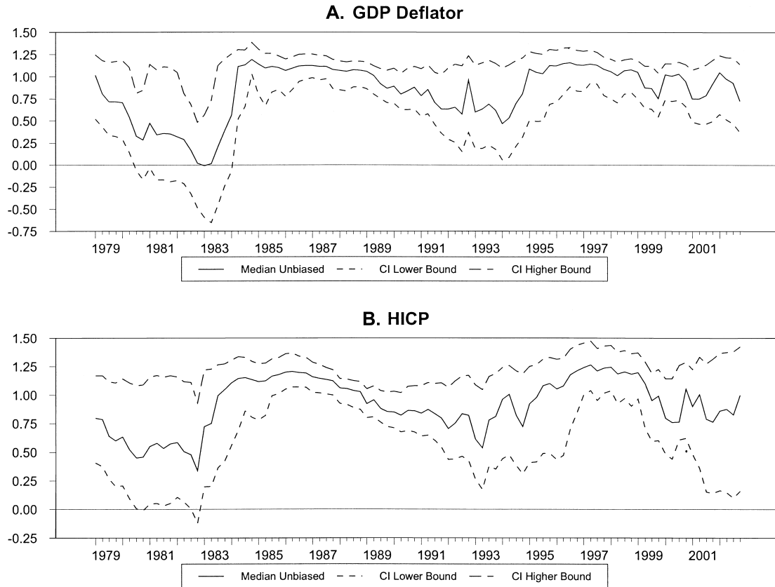
FIGURE 5.—ROLLING 8-YEAR GRID-BOOTSTRAP ESTIMATES OF \rho (WITH 90% CONFIDENCE INTERVALS)
