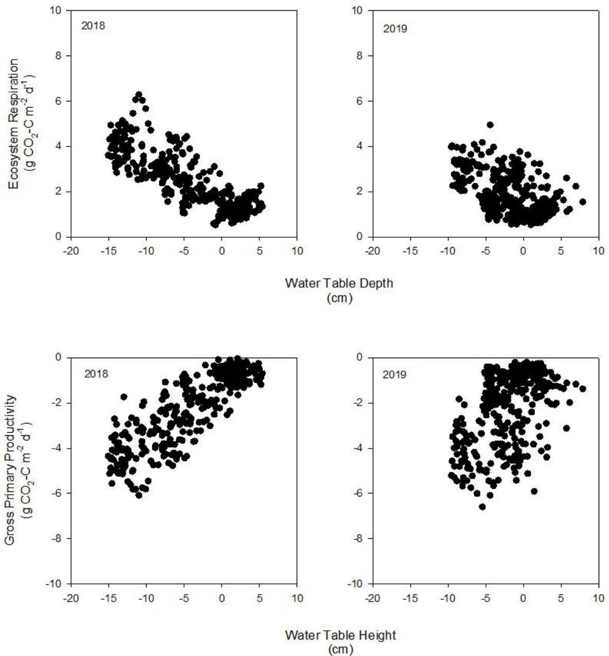
Figure 4.13. The relationship between mean daily water table height (WTH) at the central ecotone and the components of net ecosystem carbon exchange in both 2018 and 2019. The upper panels show the relationship between WTH and R_{eco} in both years, while the lower panels show the relationship between WTH and GPP in both years.
