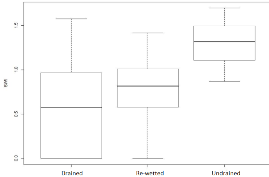
Figure 3.6.4. Boxplot of Shannon Weiner Index (SWI) values at each sampling point according to the management type at that point (drained, re-wetted, undrained).
