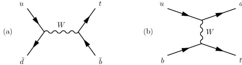
Fig. 1. LO Feynman diagrams for single top quark production via the s -channel and t -channel process.
