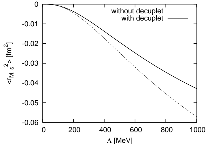
Fig. 2. Strange magnetic radius squared with (solid) and without (dashed) inclusion of decuplet loops.
