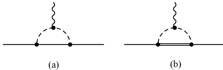
Fig. 1. Feynman diagrams contributing to the strange magnetic radius at \mathcal{O}(p^3) . Solid lines are octet baryons, dashed lines are pseudogoldstone bosons and double lines are decuplet baryons.
