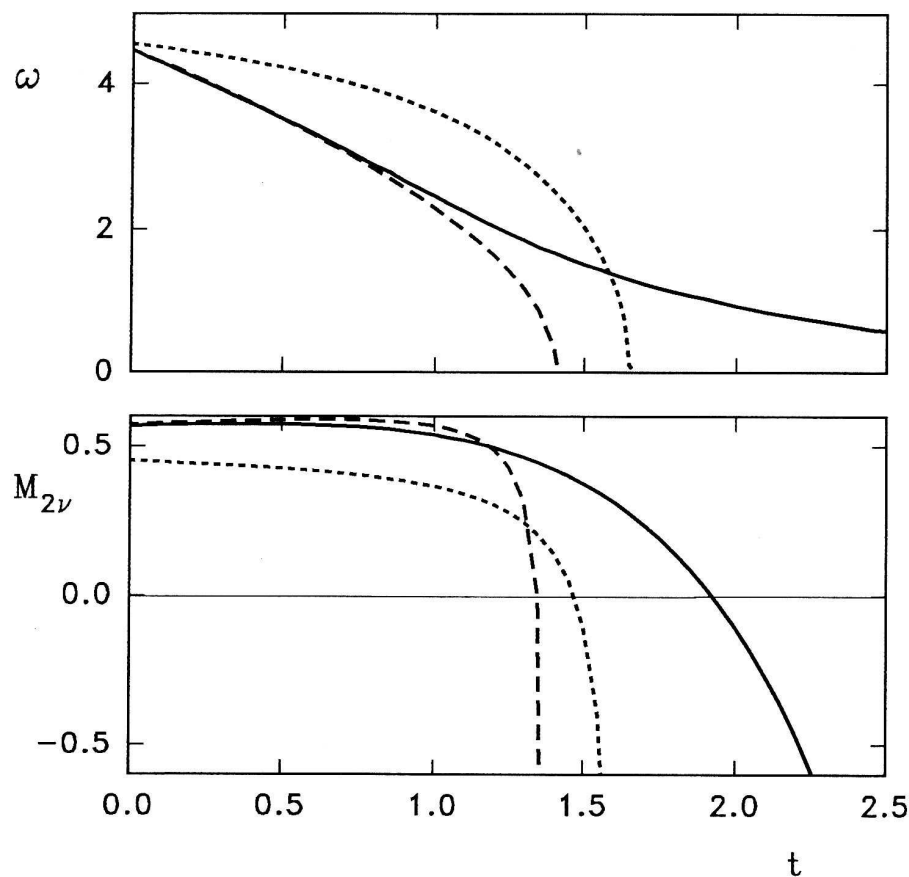
Fig. 1. Energies \omega (in MeV) of the lowest 1^+ state of ^{100}\text{Tc} and the matrix elements M_{2\nu} (in [\text{MeV}]^{-1} ) for the ^{100}\text{Mo} \rightarrow ^{100}\text{Ru} system. The single mode model results are indicated by the dashed lines for the QRPA and by the solid lines for the RQRPA. The results of a full QRPA calculation [3] are represented by dotted lines.
