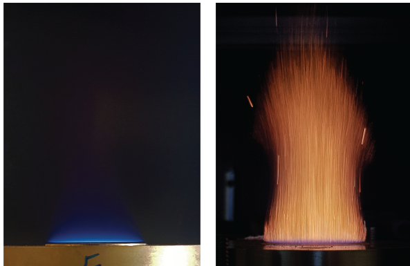
(a) Methane flame produced by the HFB with \phi_{CH_4} = 1 , v_g = 36 cm/s (b) Typical hybrid flame produced by the HHFB with \phi_{CH_4} = 1 , v_g = 35 cm/s and C_{Fe} = 22 g/m 3
