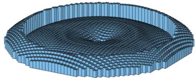
Fig. 3. The 3-D model of designed phase modulated zone plate with the relative permittivity of ~2.75.
