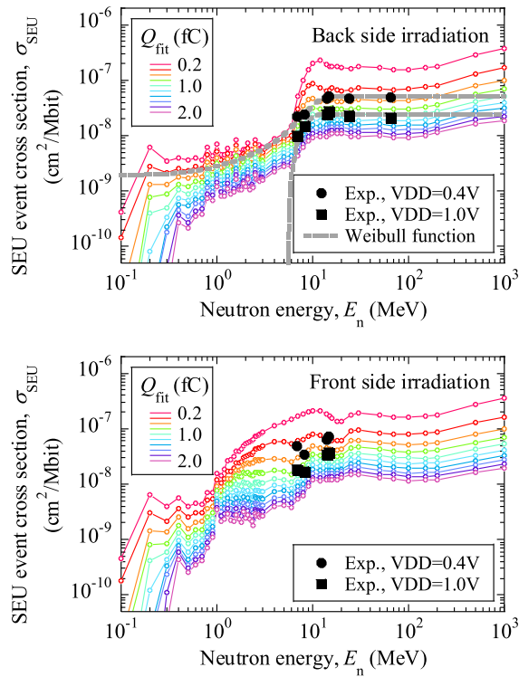
Fig. 3. SEU cross sections for various values of Q_{fit} calculated by PHITS + MSV. Irradiation of mono-energetic neutrons from the backside and frontside of DUT was simulated. Measured data are taken from [10].
