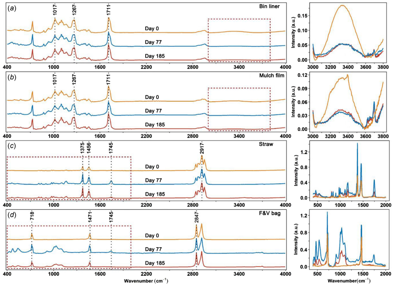
Fig. 2. ATR-FTIR spectra of original plastics and incubated plastics removed from soils after 77 and 185 days of soil incubation at 37 \pm 1^\circ\text{C} : (a) bin liner, (b) mulch film, (c) straw and (d) F&V bag. The enlarged regions of the spectra (specified with red rectangle), where substantial changes in absorption bands were observed, are presented on the right-hand side of the figure.
