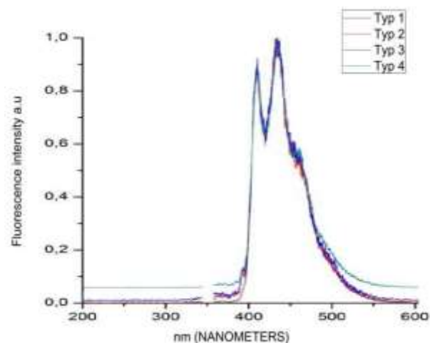
Fig. 3. Spectra of four types of collagen dissolved in xylene; typ 1, 2, 3, 4 – numbers of collagen type
