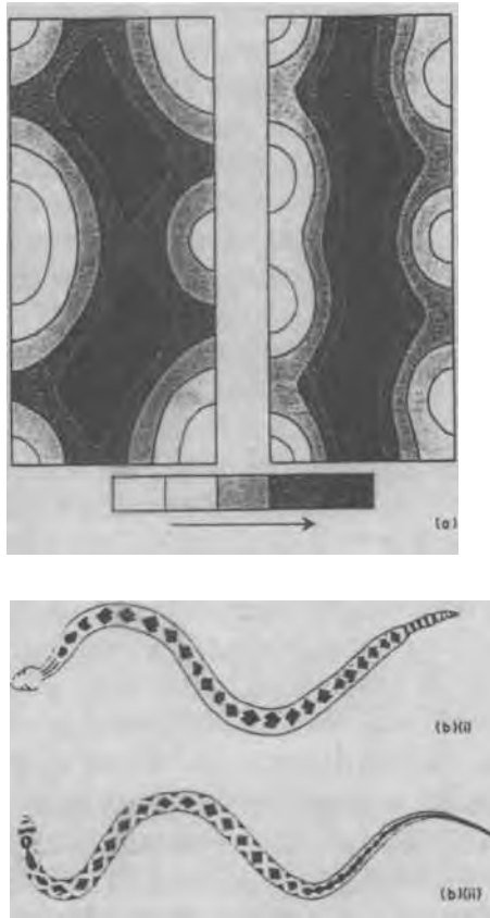
Figure 1. (a) Simulation of the cell-chemotaxis model (8)-(9) showing the effect of domain size on cell density concentration (arrow denotes increasing cell density). As the domain narrows, the diamond pattern changes to a simpler, wavy stripe pattern. This is an example of a developmental constraint, (b) Examples of diamond patterns on snakes (i) Crotalus adamanteus ; (ii) Coluber hippocrepis (note the effect of the tapering domain). (Reproduced from Murray and Myerscough, 1991, with permission).
