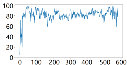
Fig. 10: Global testing accuracy in Forest CoverType.
