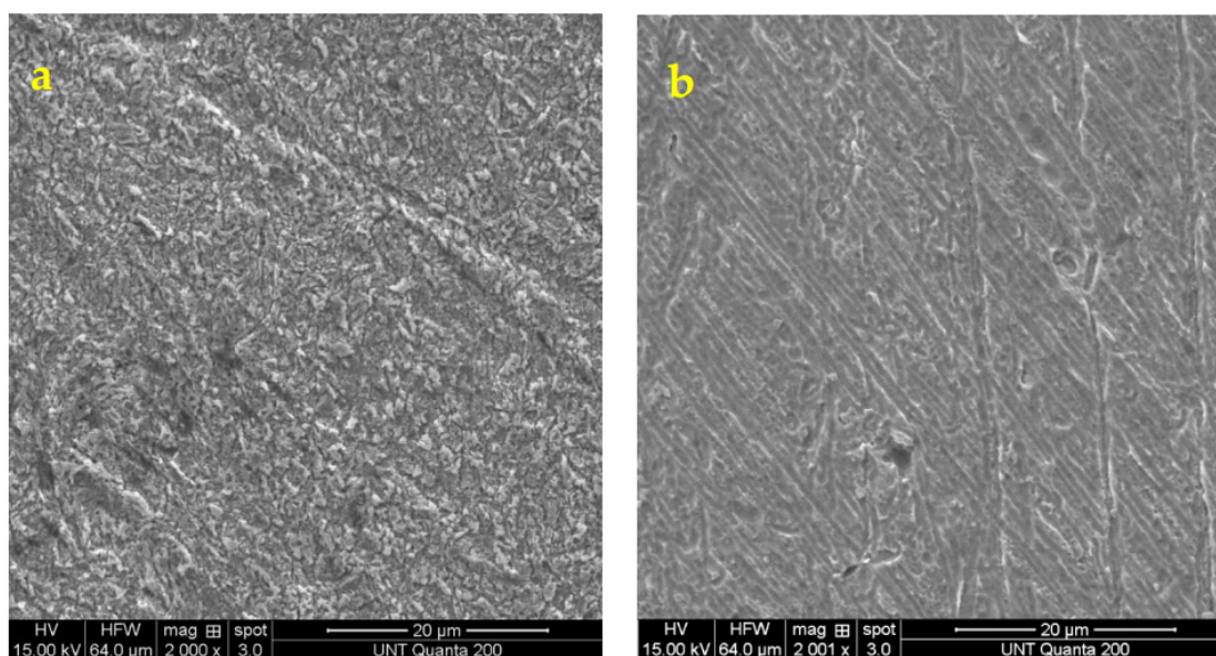
Figure 4. SEM images of brass after immersion in 0.5 M H_2SO_4 solution (a) without any inhibitor for 24 h, 2000 \times magnification and (b) with 0.25 mM of inhibitor for 24 h, 2000 \times magnification.
