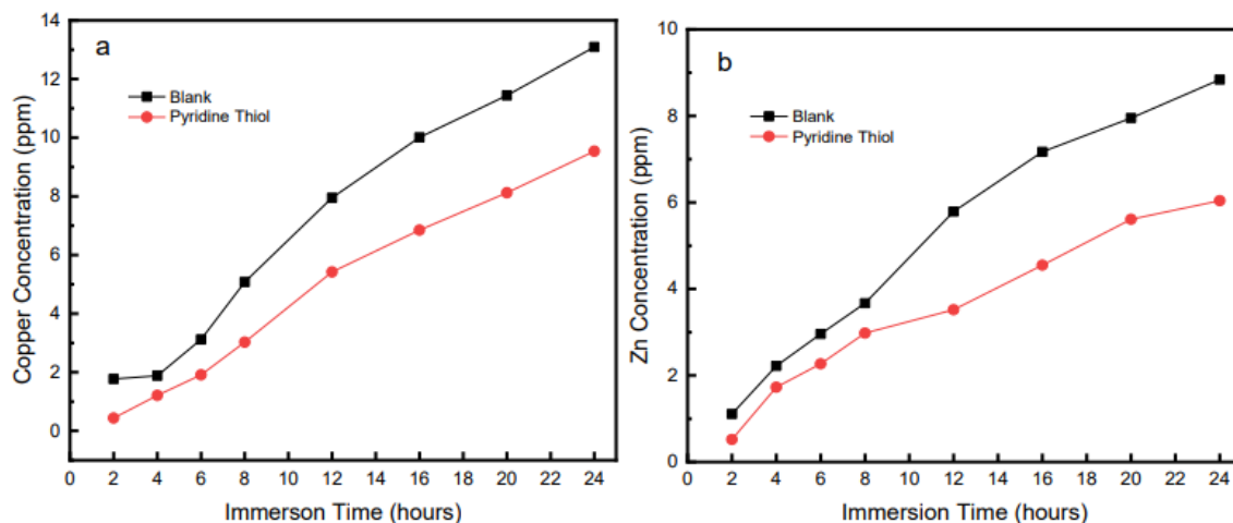
Figure 2. Copper (a) and Zinc (b) concentration (ppm) present in 0.5 M H 2 SO 4 solution with respect to immersion time for 0.5 mM P2T obtained by atomic adsorption spectroscopy measurements.
