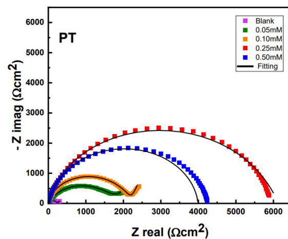
Figure 6. Nyquist plots of brass samples with and without different concentrations of corrosion inhibitors in 0.5 M H_2SO_4 .
