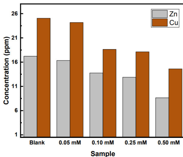
Figure 3. Copper and Zinc concentrations after an immersion time of 48 h in 0.5 M H_2SO_4 .
