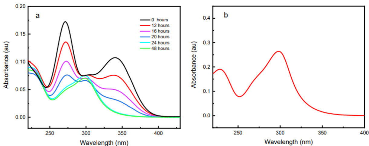
Figure 14. UV-vis spectroscopy of (a) P2T inhibited immersion solution over different time intervals and (b) UV-Vis spectrum of pure dipyridyl disulfide in 0.5 M H 2 SO 4 solution.
