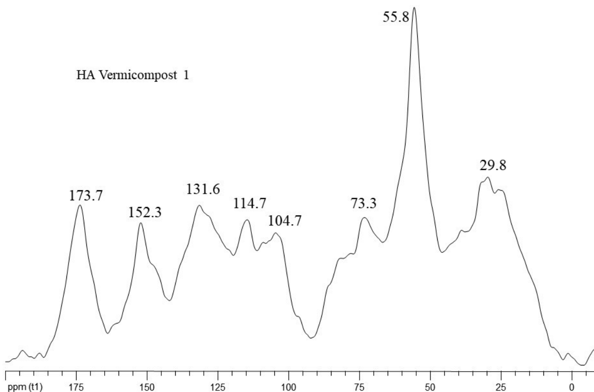
Figure 1 - 13 C NMR spectrum of humic acids isolate from vermicompost.
