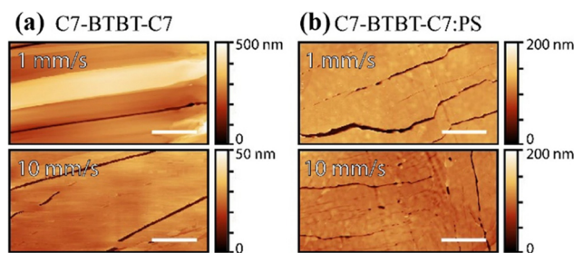
Fig. 8 AFM height image of bottom gate/top contact devices of (a) C7-BTBT-C7 and (b) C7-BTBT-C7:PS thin films deposited via BAMS at different shearing rates ( 1 \text{ mm s}^{-1} and 10 \text{ mm s}^{-1} ). The scale bar corresponds to 10 \mu\text{m} .
