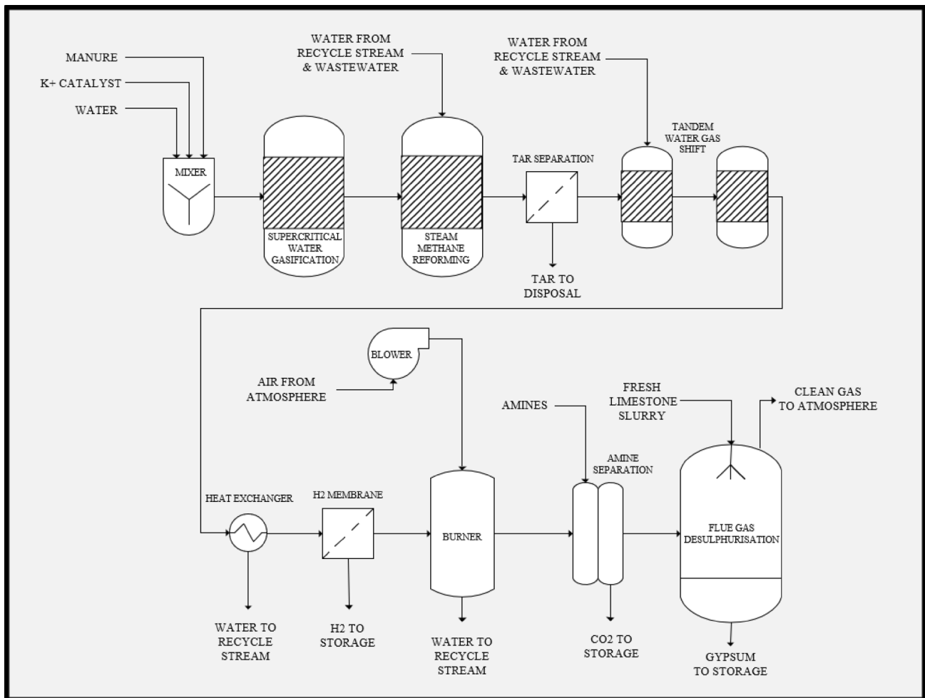
Fig. 7 Proposed schematic of a Supercritical water gasification process using manure as a feedstock. Modified from [208]
