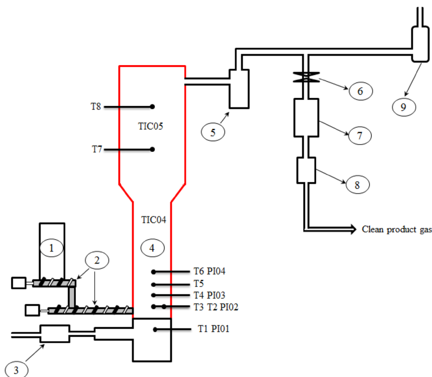
(1) biomass hopper (2) feeding screws (3) air preheater (4) gasifier reactor (5) cyclone (6) valve (7) hot filter (8) cold filter (9) flare.
