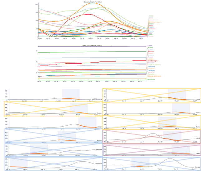
Figure 4: The time series of the target region (the top left plot), and the set of top N search results as the initial set of reference time series. The matching pattern in each time series is highlighted with the N + 1 plots organized vertically in the order of similarity to help users assess the suitability of individual reference time series for prediction.
