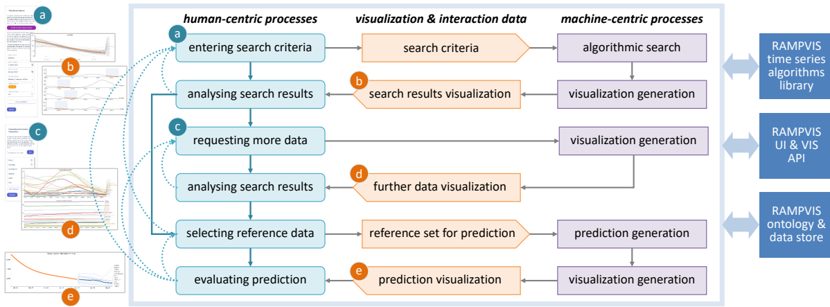
Figure 2: An overview of a typical VASAP workflow of the search-analyze-forecast tasks and how they relate to the components of the RAMPVIS infrastructure, including the time series algorithm library, UI and VIS API, ontology, and data store. The letters match the process step and with the visualization designed to support it.
