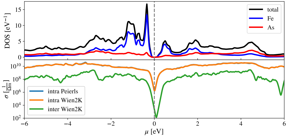
Figure 14: Hybridization-gap semiconductor \text{FeAs}_2 . Result of a WIEN2K calculation using the PBE exchange-correlation potential and 20 \times 20 \times 40 \mathbf{k} -points. (top) total and partial density of states (DOS); the DOS around the gap ( \Delta = 0.275\text{eV} ) is dominated by Fe-character. (bottom) LINRETRACE intra- and inter-band conductivities in the x -direction and as a function of the chemical potential \mu . The Peierls approximation to the optical elements leads to intra-band results (blue) virtually indistinguishable to using the full dipole matrix elements (yellow): For the given temperature ( T = 300\text{K} ) and scattering rate ( \Gamma = 10^{-5}\text{eV} ) the intra-band contributions largely dominate over inter-band effects (green).
