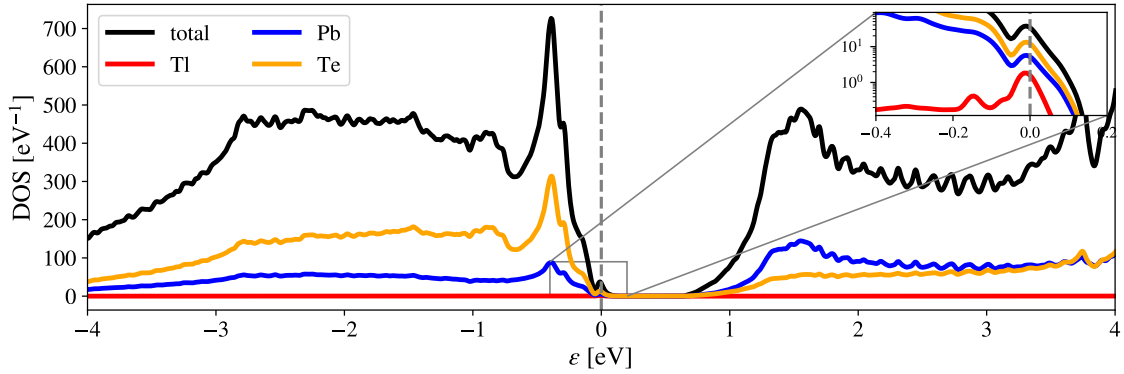
Figure 17: Tl-doped PbTe: Density of states using the LDA exchange-correlation potential and 17 \times 17 \times 17 \mathbf{k} -points. Introducing a single \text{Tl} \leftrightarrow \text{Pb} substitutional impurity results in a distorted electronic structure and additional states appear near the valence-band edge, pinning the chemical potential. The zoomed inset illustrates the non-trivial nature of the resonance to which all three elements contribute in some part.
