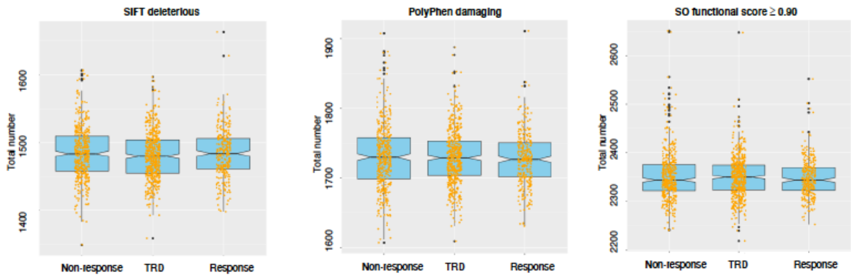
Figure 1: representation of exome-wide distribution of variants with Sequence Ontology (SO) functional score \geq 0.90 , SIFT deleterious variants, PolyPhen damaging/probably damaging variants. The examined phenotypic groups (x axis) were treatment-resistant depression (TRD), non-response and response. The number of variants in each phenotypic group is reported on the y axis.
