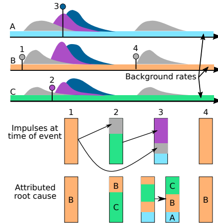
Figure 8: Representation of a Hawkes model with three processes. Events cause impulses that increase the rate of subsequent events in the same or other processes. By looking at the impulses present when events occur, the probability of a process being the root cause of an event can be determined. Note that on the second part of the Figure, colors represent events while arrows represent impulses between the events.
