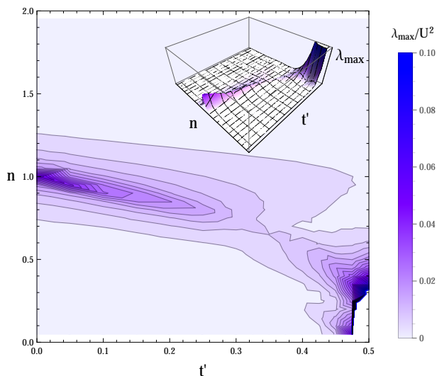
FIG. 8. Plot of highest effective coupling constant \lambda_{max} irrespective of type of wave. Inset shows a 3D version of the same plot. Clear maxima can be seen at the FM and AFM point as well as an increase in coupling strength in the vicinity of the Van Hove line.
