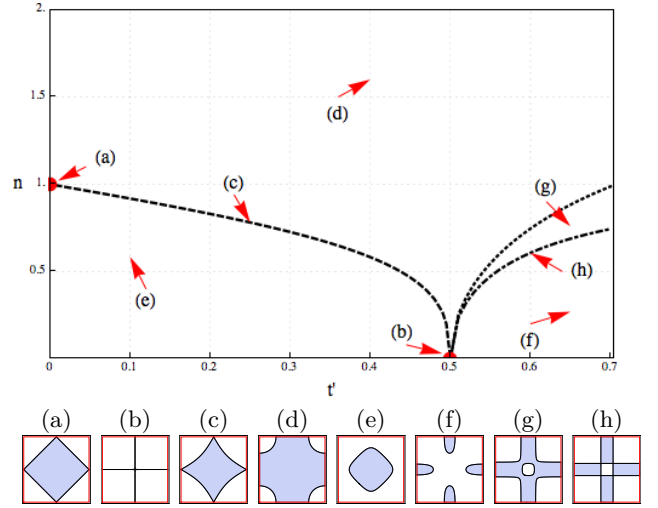
FIG. 4. The parameter space of 0 \leq n \leq 2 and 0 \leq t' \leq 0.7 is plotted. The Van Hove line (dashed), second line of nesting (dot-dashed) and line beneath which a Fermi pocket exists (dotted) are portrayed. The position and characteristic Fermi surfaces in the first Brillouin zone (of size k_x, k_y \in (-\pi, \pi) ) are shown for: (a) the antiferromagnetic point \{n=1, t'=0\} , (b) the ferromagnetic point \{n=0, t'=0.5\} , (c) an arbitrary point along the Van Hove line \{n=0.78, t'=0.25\} (d), above the Van Hove line \{n=1.60, t'=0.4\} , (e) below the Van Hove line \{n=0.58, t'=0.1\} , (f) below the second nested line \{n=0.27, t'=0.65\} , (g) above the second line of nesting, in a region where a Fermi pocket exists around (k_x, k_y) = (0, 0) \{n=0.76, t'=0.65\} , (h) on the second line of nesting \{n=0.61, t'=0.6\} .
