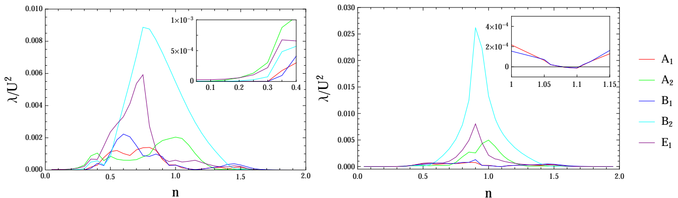
FIG. 7. left : Line at t' = 0.3 for 0 < n < 2 . The highest value for \lambda corresponds to the Van Hove density n_{vh} \approx 0.726 . The inset shows the leading harmonics at low fillings ( 0.05 \leq n \leq 0.4 ). right : line at t' = 0.1 for 0 < n < 2 . The highest value for \lambda corresponds to the Van Hove density n_{vh} \approx 0.918 . The inset shows negative values for the A_1 and B_1 representations for 1.08 \leq n \leq 1.11
