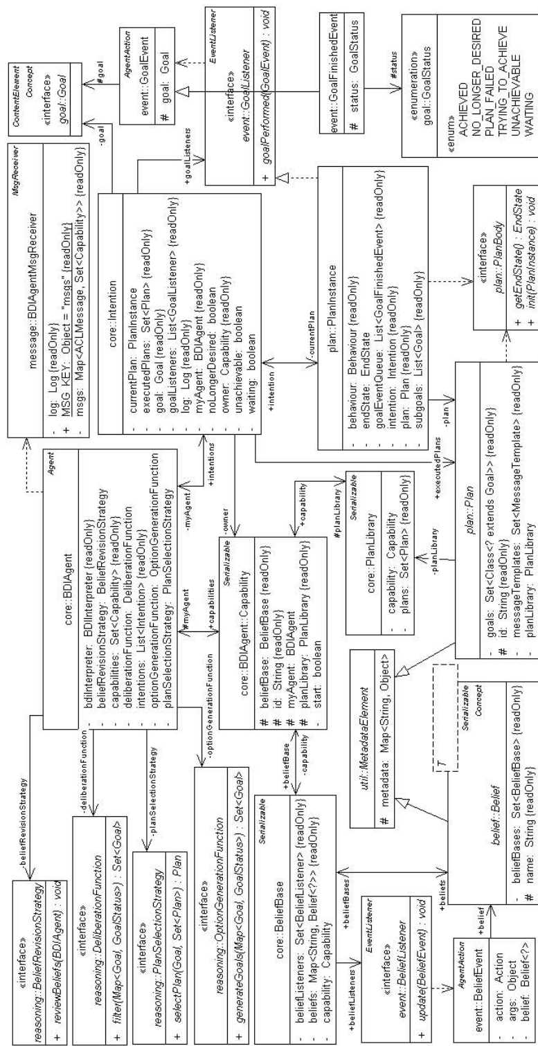
Fig. 1: Class diagram – BDI4JADE main classes and interfaces.
