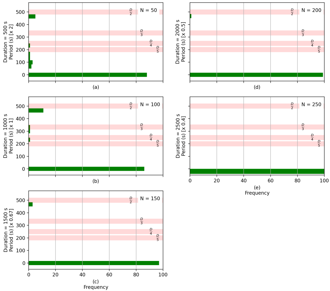
Figure 5.3: Histograms of statistically significant IMF periods from 100 samples of with constant cadence of 10 s, and varying duration, D , and therefore number of datapoints N , with N = 50 (a), N = 100 (b), N = 150 (c), N = 200 (d), and N = 250 (e). All vertical axes of the histograms have been rescaled to match (b) so that results can be directly compared. Red shaded regions indicate the expected locations of overtones \frac{D}{2} , \frac{D}{3} , \frac{D}{4} , and \frac{D}{5} .
