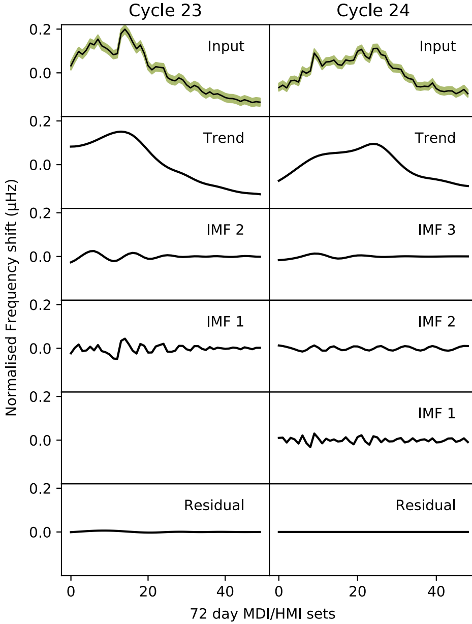
Figure 4.2: Averaged frequency shifts from modes with lower turning points between 0.7\text{--}0.75 R_{\odot} and frequency between 3200\text{--}3600 \mu\text{Hz} during Cycle 23 ( Top left ) and Cycle 24 ( Top Right ) as measured by MDI/HMI. Frequency shifts have been normalised to have zero mean, with errors seen in green. Lower panels show the IMFs obtained from the decomposition from Cycles 23 ( Left ) and 24 ( Right ). IMF 2 (with an average period of 721 d) from Cycle 23 and IMFs 2 (437 d) and 3 (889 d) from Cycle 24 are statistically significant above a 95% confidence level. The IMFs with the shortest average periods from each cycle, (IMFs 1) are excluded from the analysis as they cannot be assessed with the confidence levels used.
