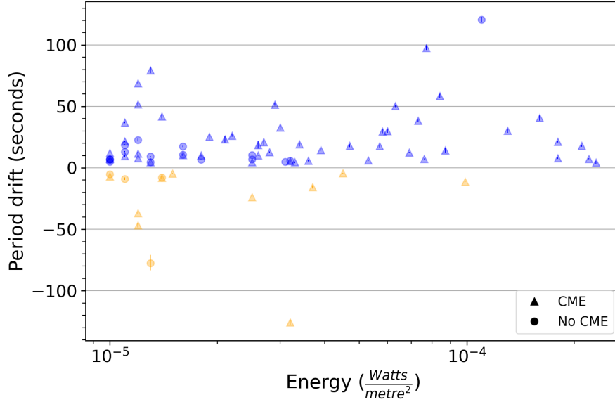
Figure 7.11: Peak flare energy as measured in GOES 1 – 8 Å plotted against QPP period drift with no correlation. The meanings of colours and symbols are as given in Fig. 7.10.
