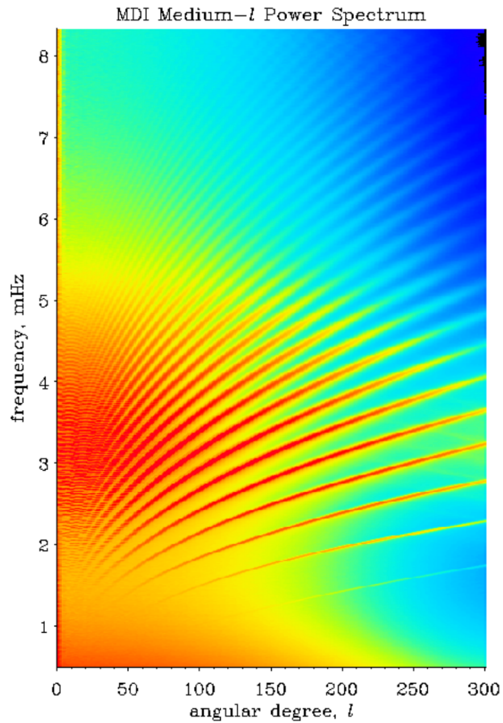
Figure 2.8: A l - \nu diagram of frequency versus harmonic degree, produced by 2 months of intermediate degree Michelson Doppler Imager data from The Solar and Heliospheric Observatory from May-June 1996. Each ridge represents a different radial order n , and spectral power density is indicated by colour. Image courtesy of NASA, see https://soho.nascom.nasa.gov/gallery/Helioseismology/
