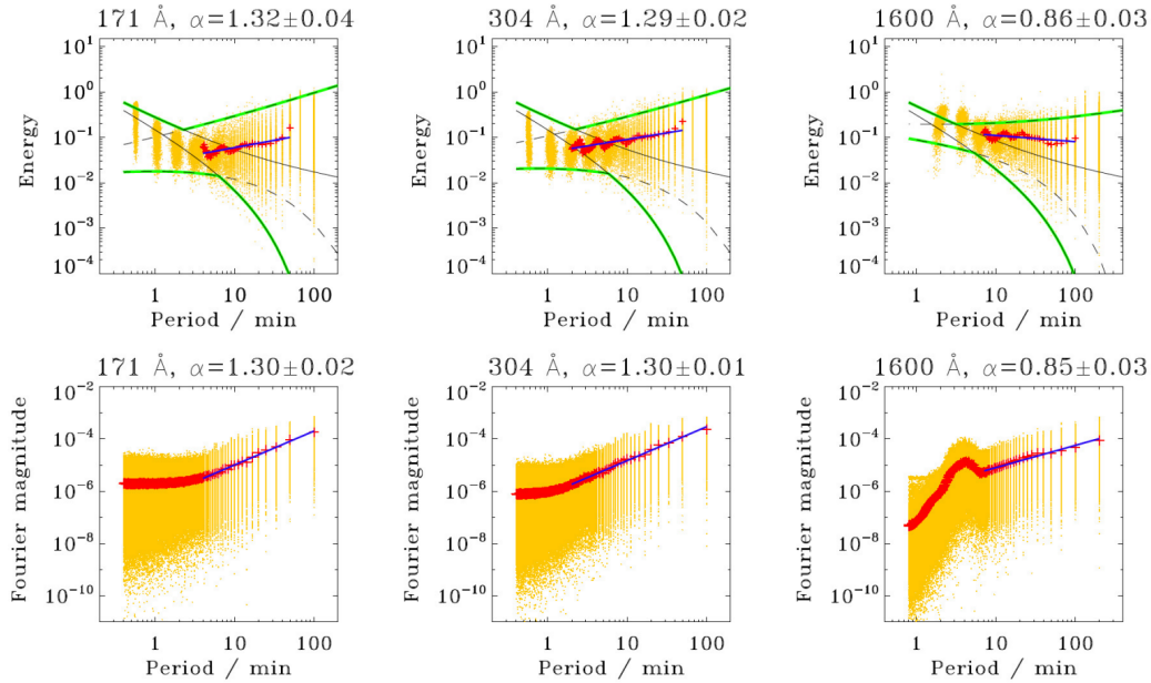
Figure 5.1: Top panels: Spectral power and periods of IMFs as yellow dots, where the IMFs have been obtained by EMD assessing SDO/AIA data from the NOAA 11131 active region from 00:00 – 03:20 UT on 8 th December 2010. 99% confidence levels are shown in green and average period energy for each IMF is shown in red , with a linear fit of the mean modal energies shown in blue . Bottom panels: Fourier spectral power and periods of Fourier harmonics, again individually shown in yellow dots, with mean Fourier magnitudes shown in red and fitted linearly in blue . We see the Fourier harmonics as vertical stripes, which are analogous to EMD overtones. Figure originally produced as Fig. 4 from Kolotkov et al. [2016].
