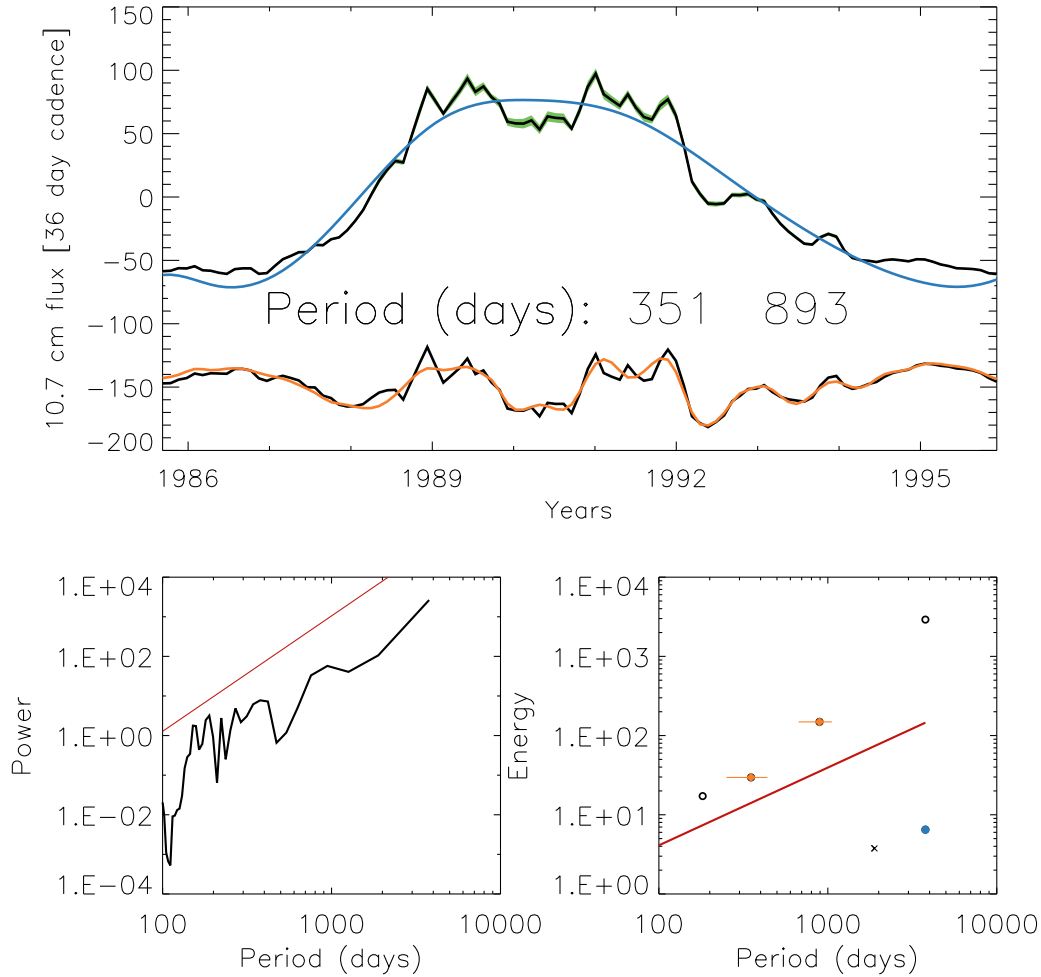
Figure 6.5: Analysis of F_{10.7} data over Cycle 22 where data is averaged over 108 d bins, overlapping by 36 d. ( Top ) Upper curve shows the normalised F_{10.7} data, with errors in green, superimposed with the IMF associated with the trend, shown in blue. Lower curve shows the detrended signal with the overlaid sum of two statistically significant IMFs. These IMFs have periods of 351^{+88}_{-100} , 893^{+163}_{-221} d. ( Lower left ) FFT spectrum of the F_{10.7} data, with 95% confidence level (solid red line). ( Lower right ) EMD spectrum of the F_{10.7} data with IMFs visualised as bullet points, indicating their average periods and spectral energy. The 95% confidence level is shown by red line. The IMF with the lowest period cannot be assessed with the confidence level given and is excluded from the analysis. Statistically significant IMFs with energy over the confidence levels are seen in orange with the error in period shown as a horizontal orange line. The IMF associated with the trend is shown in blue and the residual is indicated by a cross.
