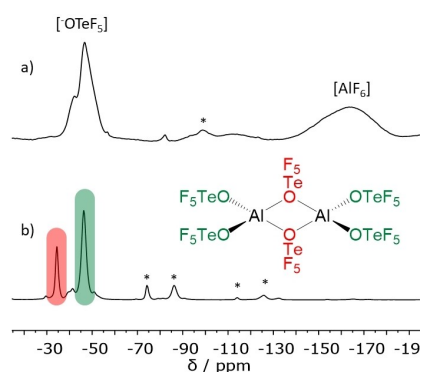
Figure 2. 19 F MAS NMR spectra for a) ACF-teflate ( \bar{\nu}_{\text{rot}} : 20 kHz) and for b) [Al(OTeF 5 ) 3 ] 2 ( \bar{\nu}_{\text{rot}} : 15 kHz). Asterisks (*) represent spinning sidebands; Lewis structure of [Al(OTeF 5 ) 3 ] 2 with bridging (red) and terminal (green) [OTeF 5 ] - groups.
