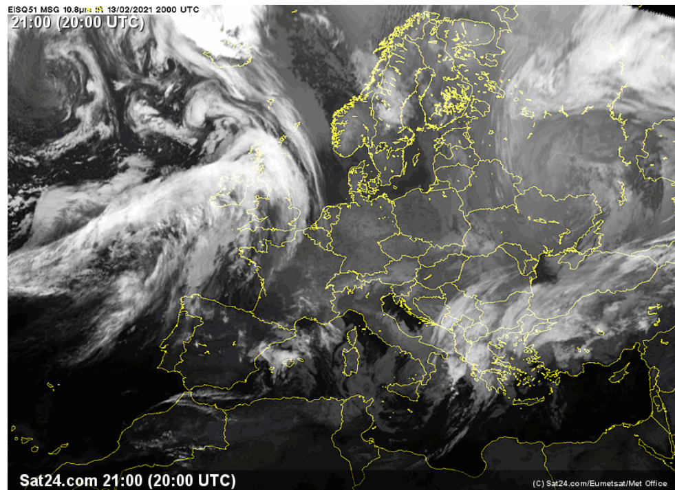
Figure 5. Infrared (10.8 \mu\text{m} ) satellite image from SAT24-EISQ51 over Europe on 13 February 20 UTC showing a clear sky over Switzerland and Germany.
