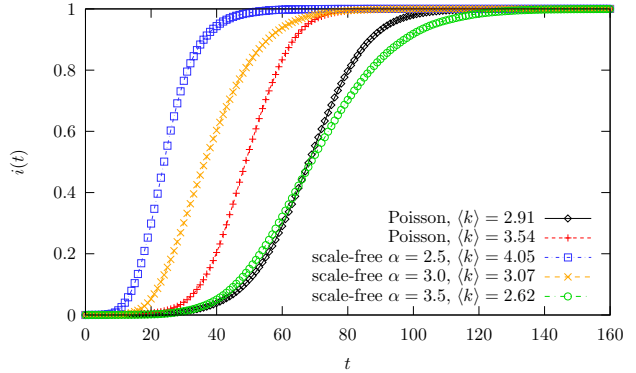
Figure 6. As in Fig. 5, but for N = 10^4 .
