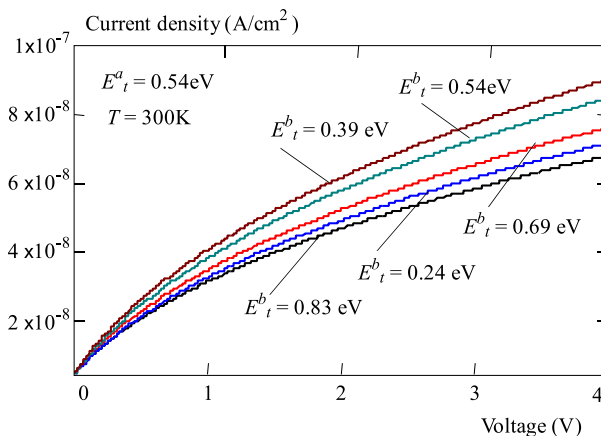
Fig. 4. Reverse I-V characteristics with CDL effect with E_t^a = 0.55 \text{ eV} and various E_t^b
