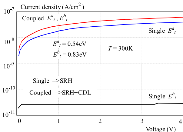
Fig. 3. Comparison of our CDL model with single SRH model of a PN diode contaminated by gold
